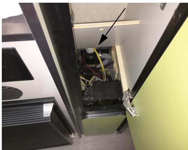
Waste Pump (Located beneath pantry cabinet - lift access panel) -Typical View
