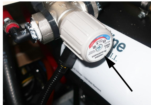
Hydronic Heating System Tempering Valve (Located below dinette seat - remove screws and panel to access) -Typical View
